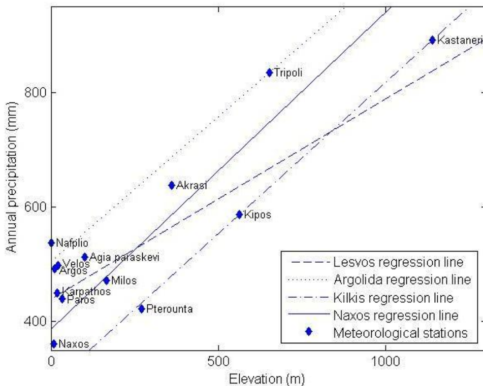
Figure 3 – Regression analysis of the precipitation data collected in the four target areas in Greece
